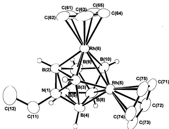
Fig. 1 The ORTEP-type drawing 9 of the crystallographically determined molecular structure of compound 2 , with the C 5 Me 5 methyl groups omitted for clarity. Selected interatomic distances (pm): Rh(6)–Rh(7) 274.75(7), N(1)–B(2) 157.5(11), N(1)–B(3) 168.6(10), N(1)–B(4) 161.5(11), N(1)–B(5) 157.0(20), N(1)–Rh(6) 306.5(9), N(1)–Rh(7) 310.8(9), B(2)–B(3) 207.8(13), B(3)–B(4) 203.1(12). The Rh–B distances are in the range 207.8(8)–220.0(9), and the B–B distances within the range 175.0(20)–180.0(14). In solution the compound has effective mirror-plane symmetry (see NMR footnote), through N(1)B(3)B(5)B(10), the mid-point of Rh(6)–Rh(7) and the mid-point of B(8)–B(9)
